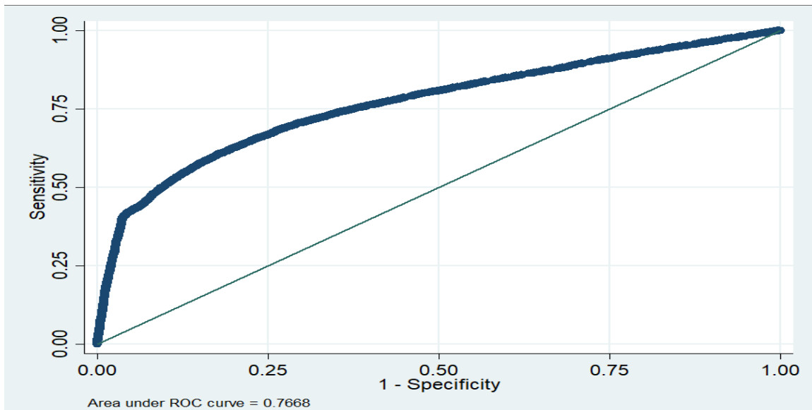
Chart 1: the ROC curve for the probit model
